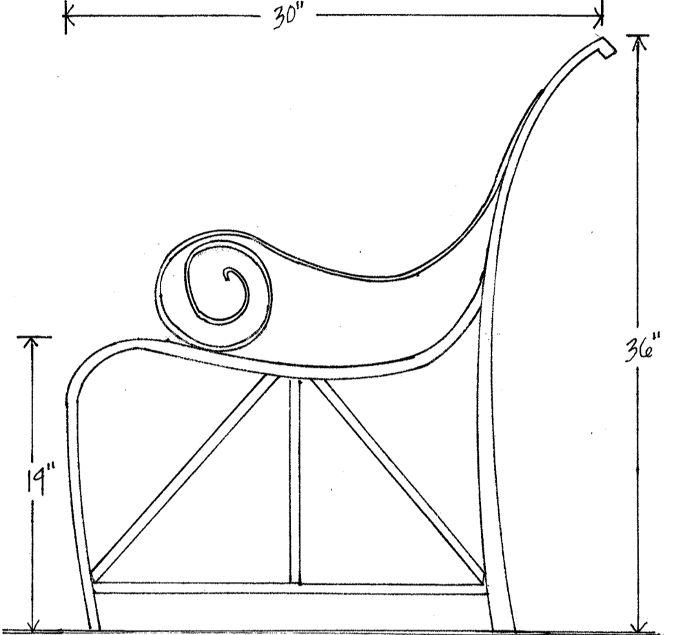
EXISTING BENCH 1/2" = 1'-0"
