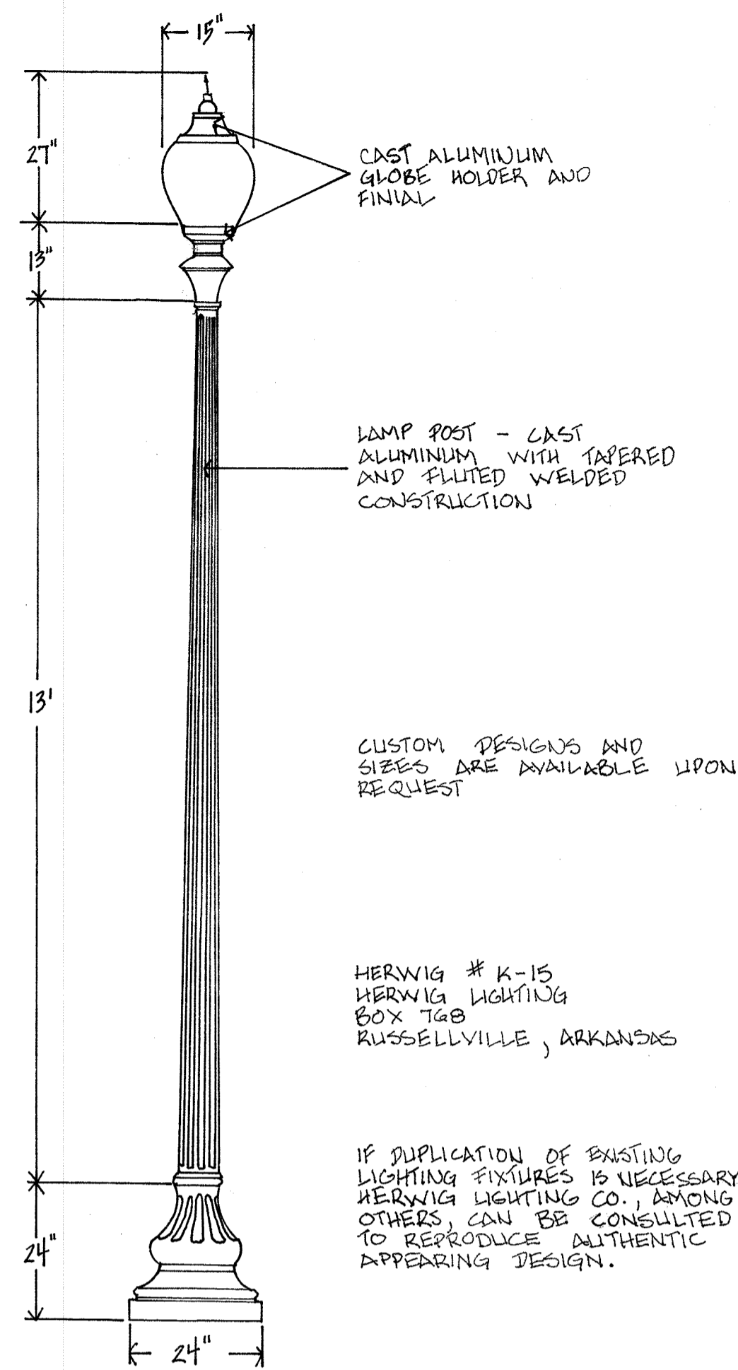
ALTERNATE FIXT. 1/2" = 1'-0"
