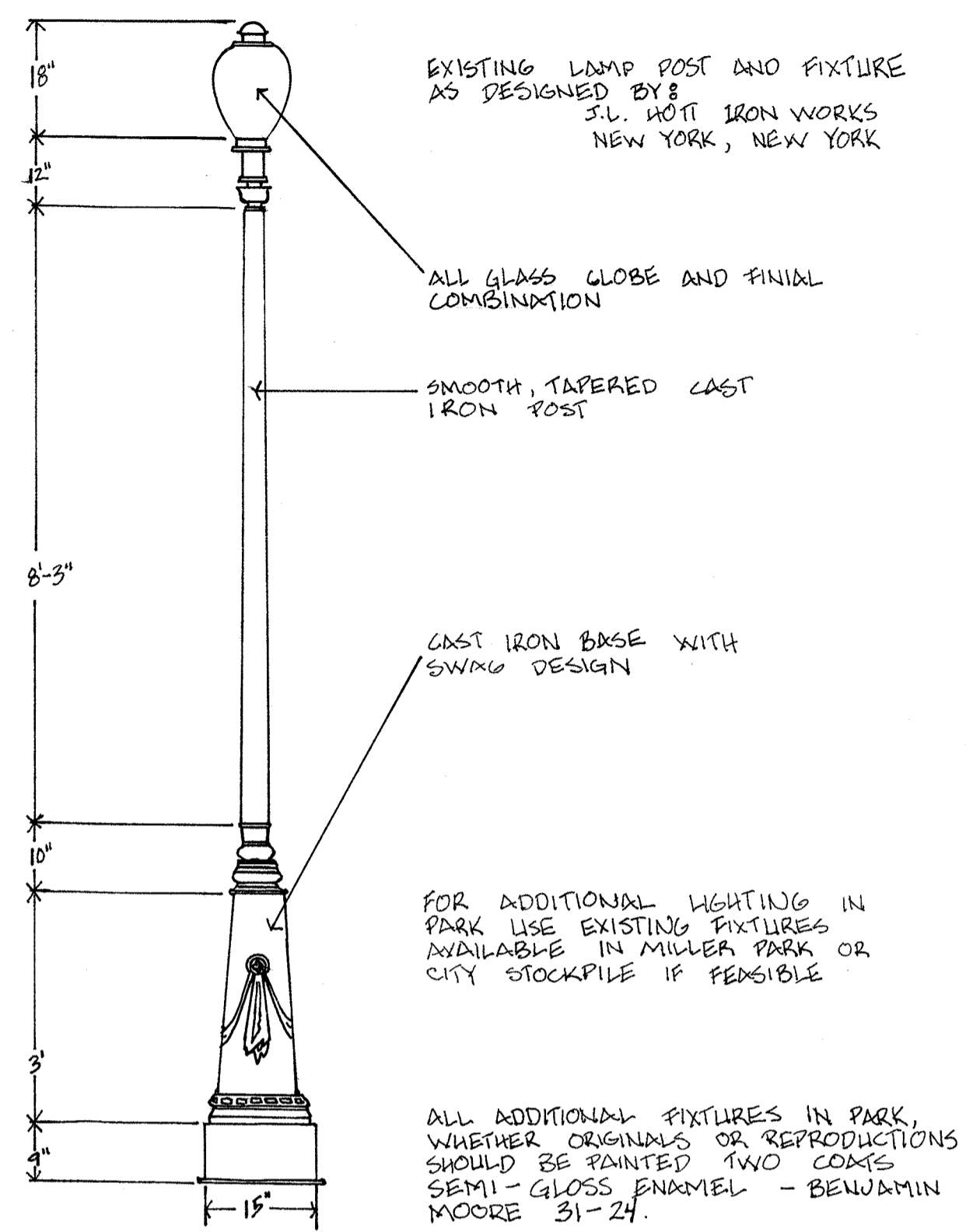
EXISTING FIXT. 1/2" = 1'-0"
