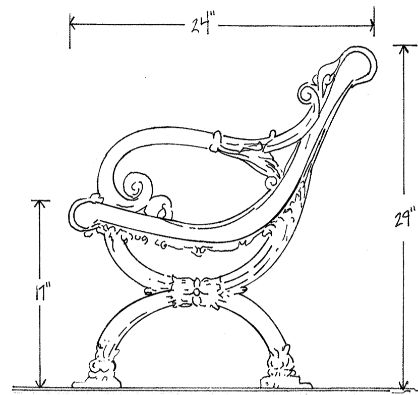
ALTERNATE BENCH 1/2" = 1'-0"
