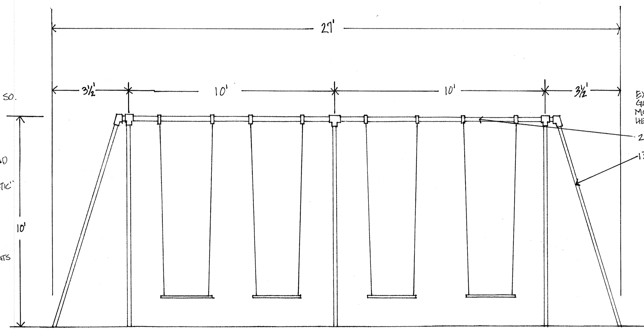
PLAYGROUND EQUIP. 3/8" = 1'-0"
